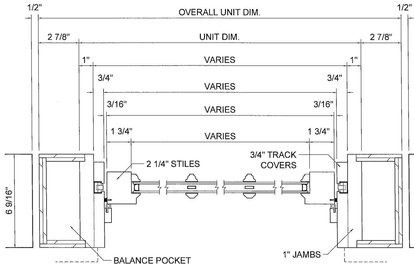
EXTERIOR ELEVATION OF SERIES 5000 INLINE FOLD-UP IN WINDOW UNIT WITH SILL
