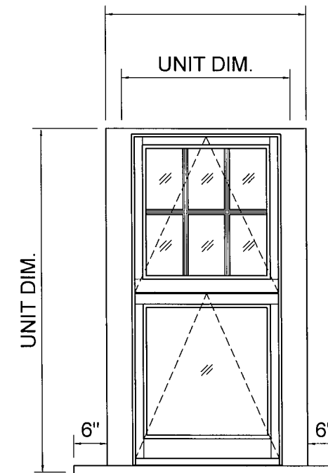
EXTERIOR ELEVATION OF SERIES 5000 INLINE FOLD-UP IN WINDOW UNIT WITH SILL
